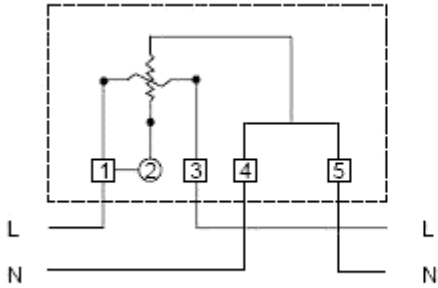
Sequential connection
