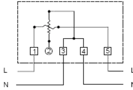
Symmetrical connection
